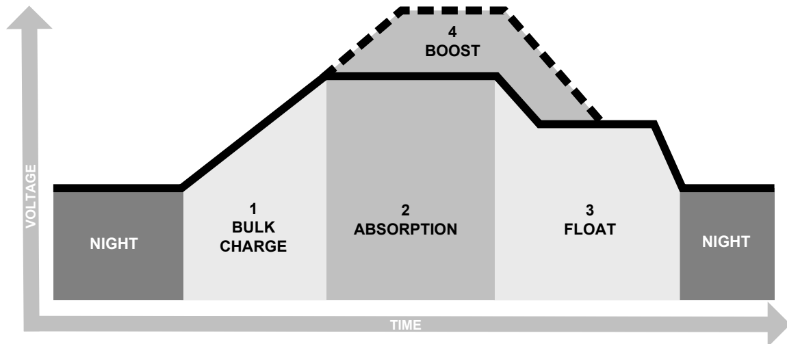
Figure 7. Algorithme de charge du SunSaver Duo
