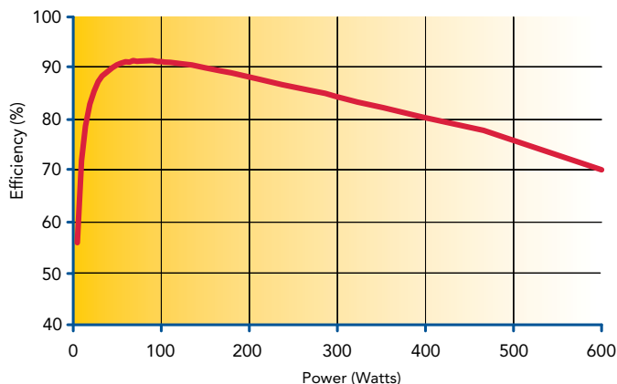
Inverter Efficiency
