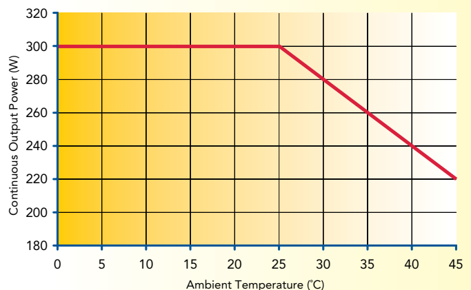
Temperature De-Rate Curve
