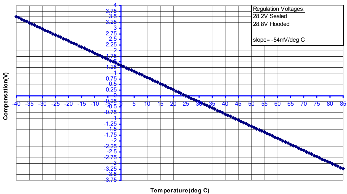
Temperature Compensation (SunLight 24V Models)
