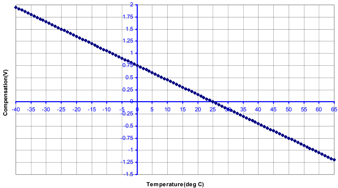
Temperature Compensation (SHS Models)
