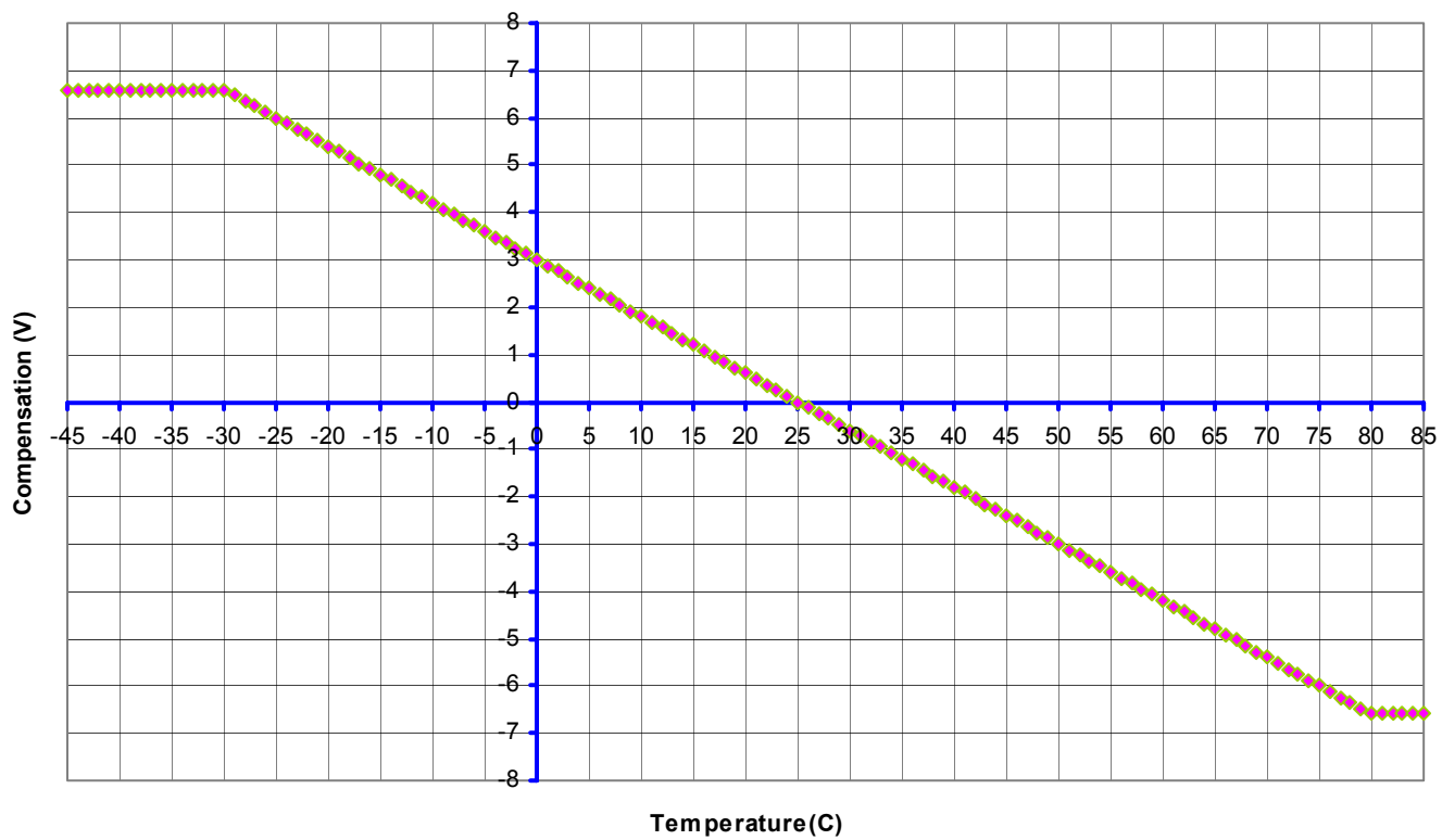
Temperature Compensation ProStar 48V
