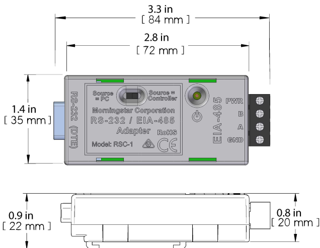
Figure 1. Dimensions RSC-1.
