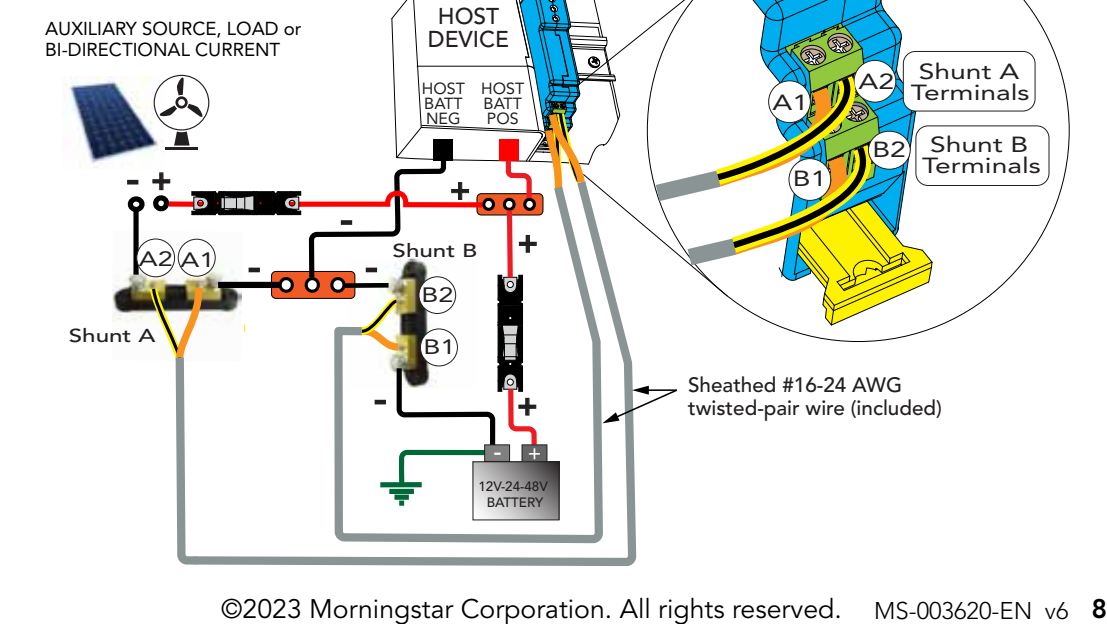
Figure 3 - Net Battery & Auxiliary Current Application
