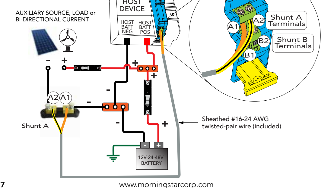
Figure 2 - Auxiliary Current Application
